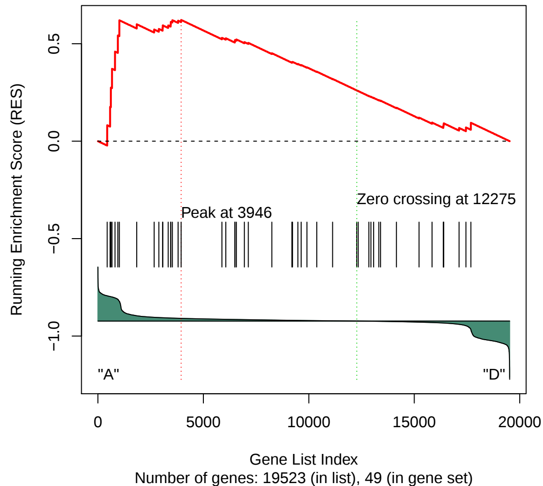
Gene Set 39 : KEGG_GLYCEROLIPID_METABOLISM
