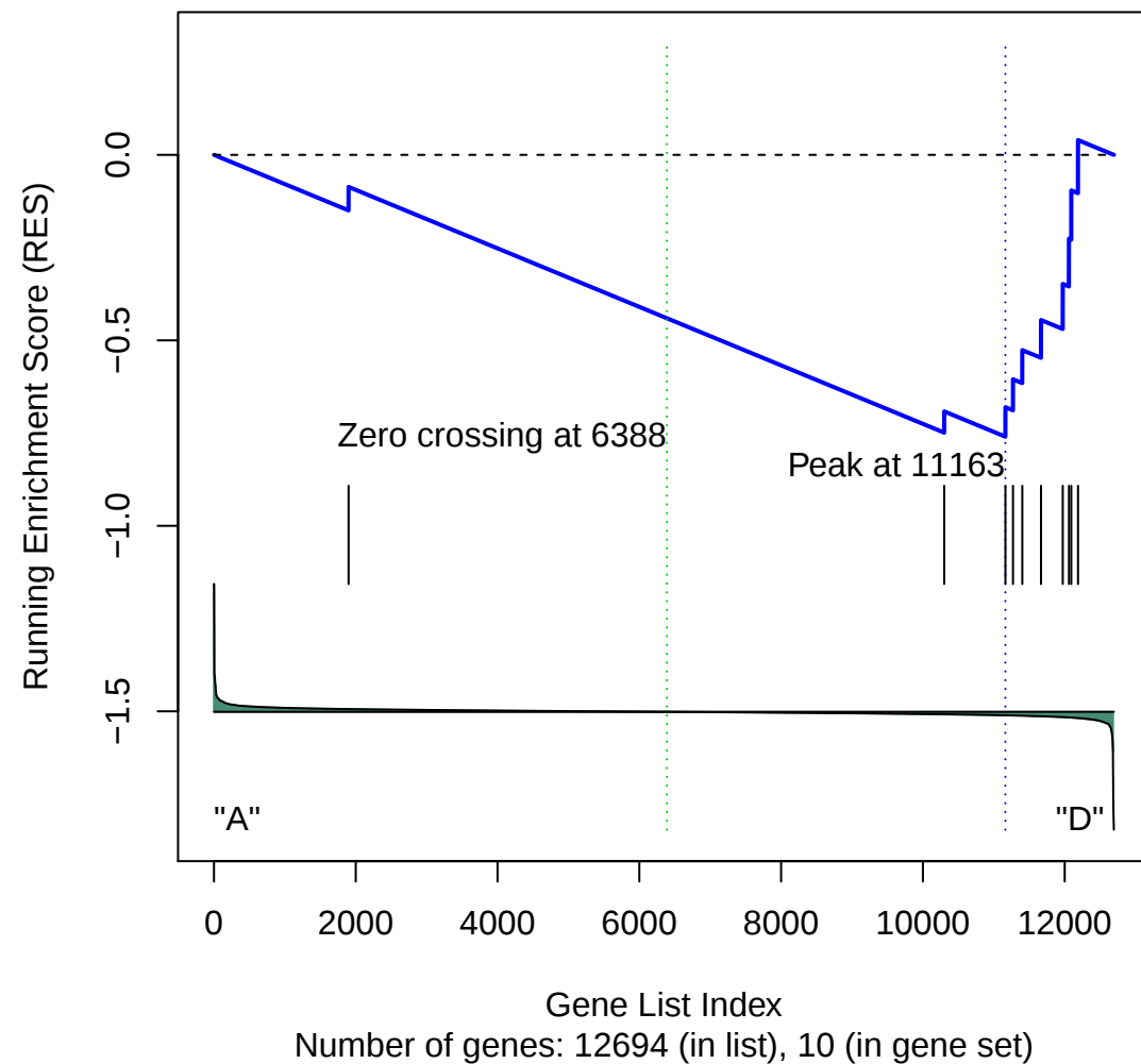
Gene Set 55 : KEGG_DNA_REPLICATION
