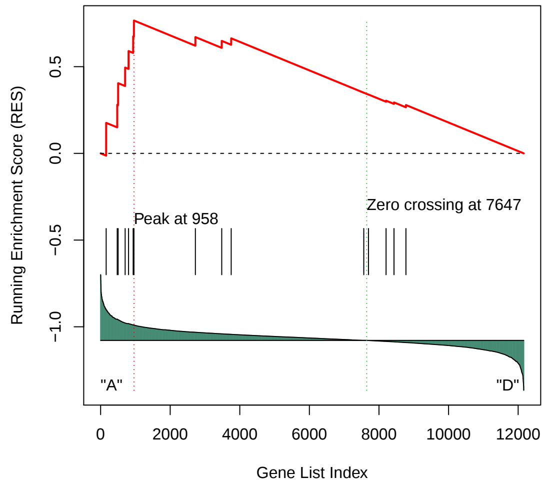
Gene Set 175 : KEGG_ALLOGRAFT_REJECTION
