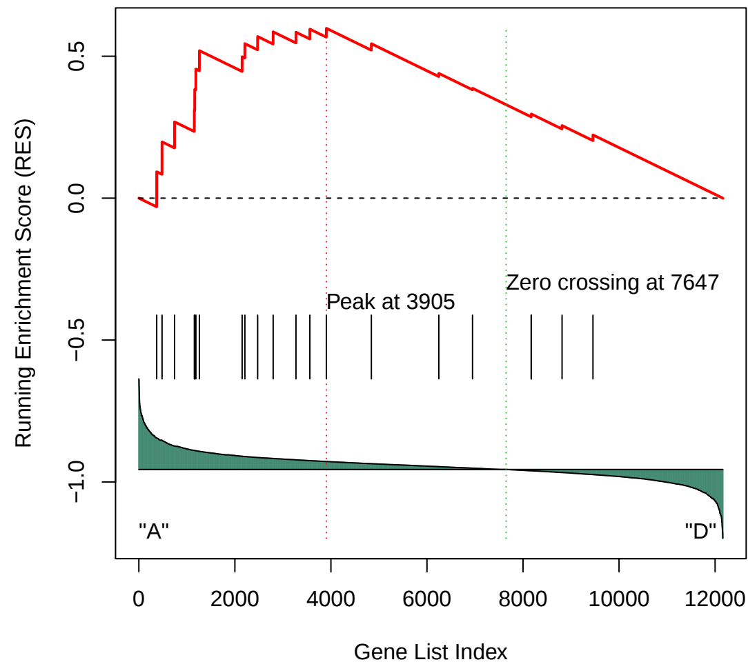
Gene Set 81 : KEGG_HOMOLOGOUS_RECOMBINATION
