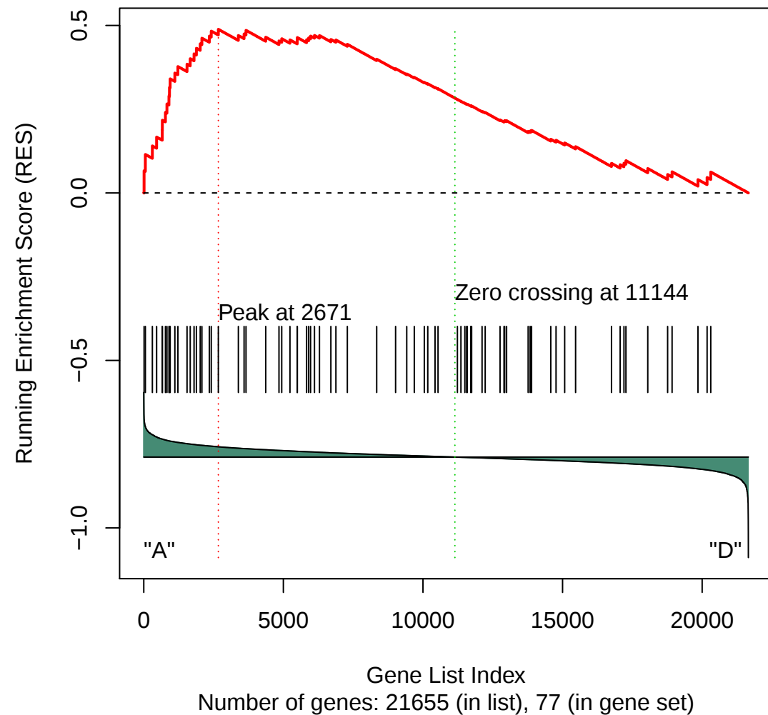
Gene Set 99 : KEGG_PEROXISOME
