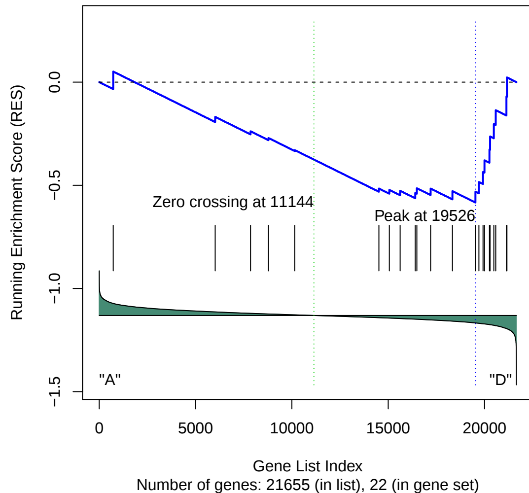
Gene Set 81 : KEGG_MISMATCH_REPAIR
