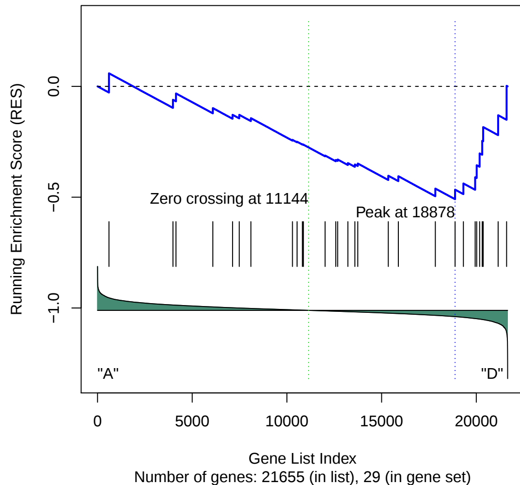
Gene Set 167 : KEGG_THYROID_CANCER
