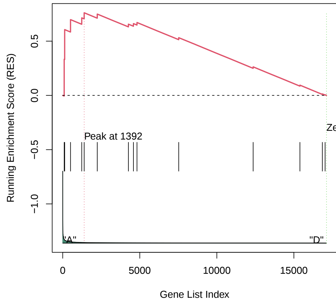
Gene Set 174 : KEGG_ALLOGRAFT_REJECTION
