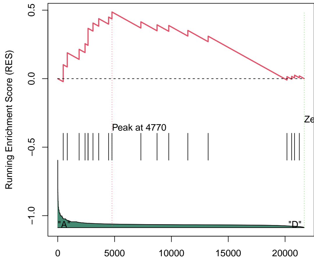
Gene Set 175 : KEGG_ASTHMA
