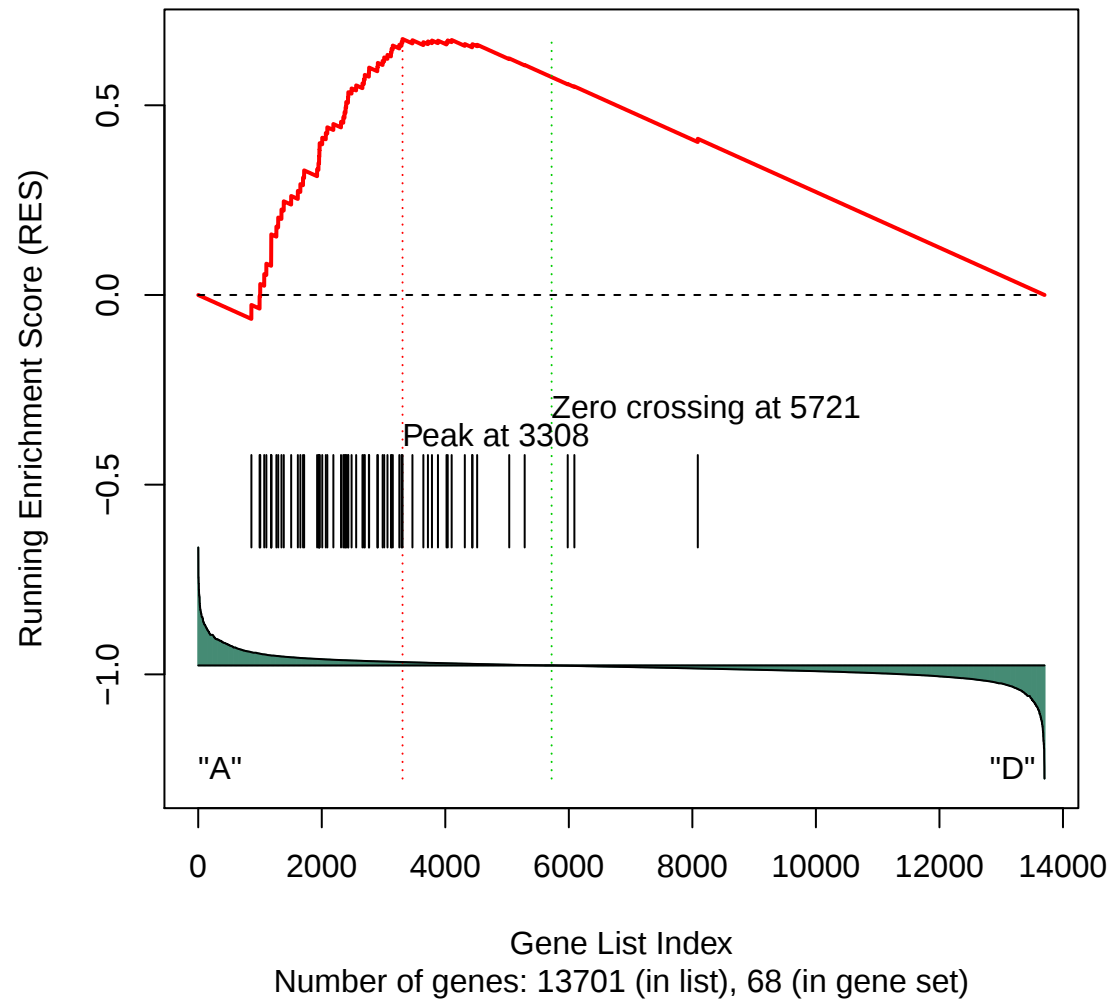
Gene Set 67 : KEGG_RIBOSOME
