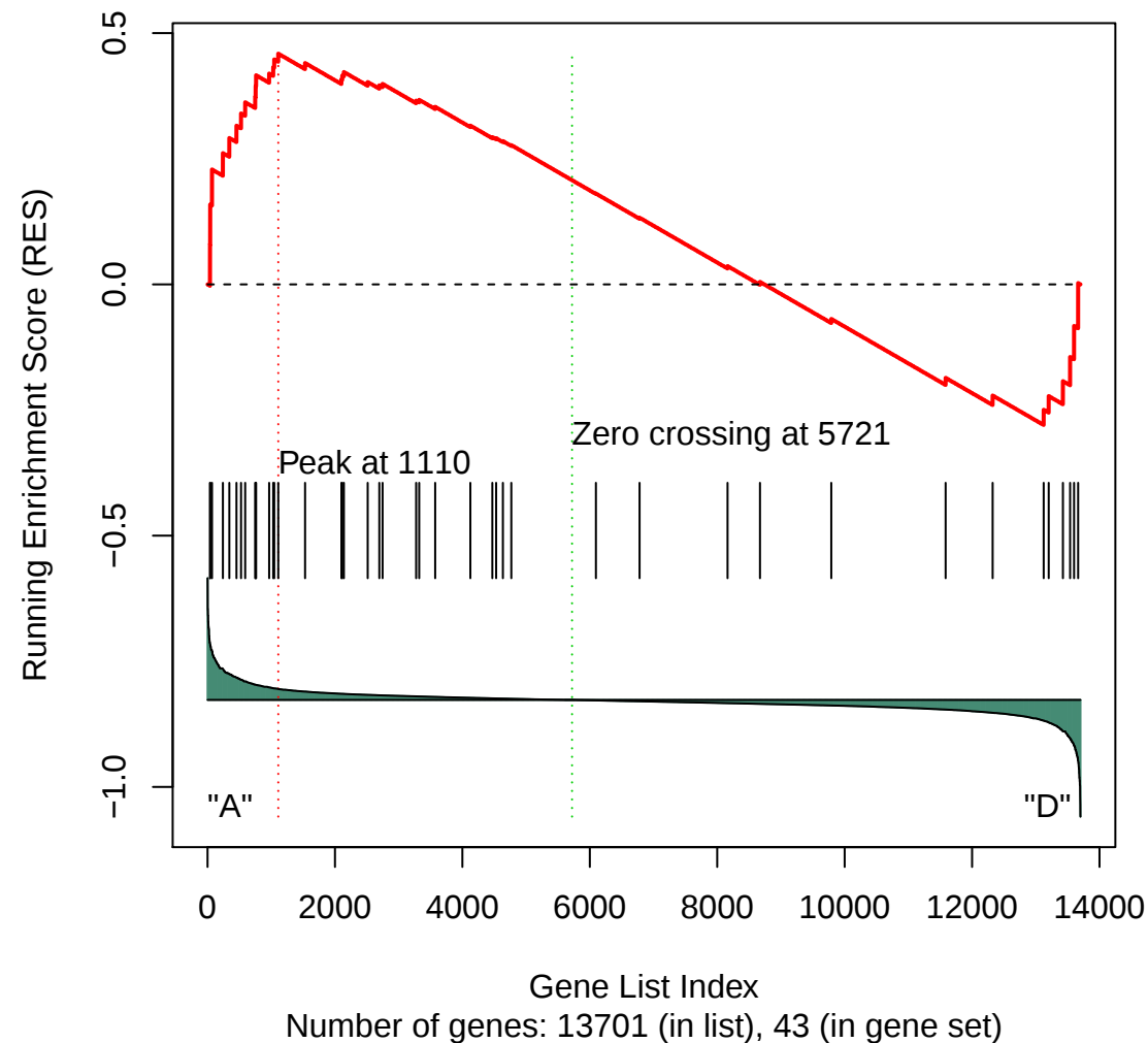
Gene Set 56 : KEGG_RETINOL_METABOLISM
