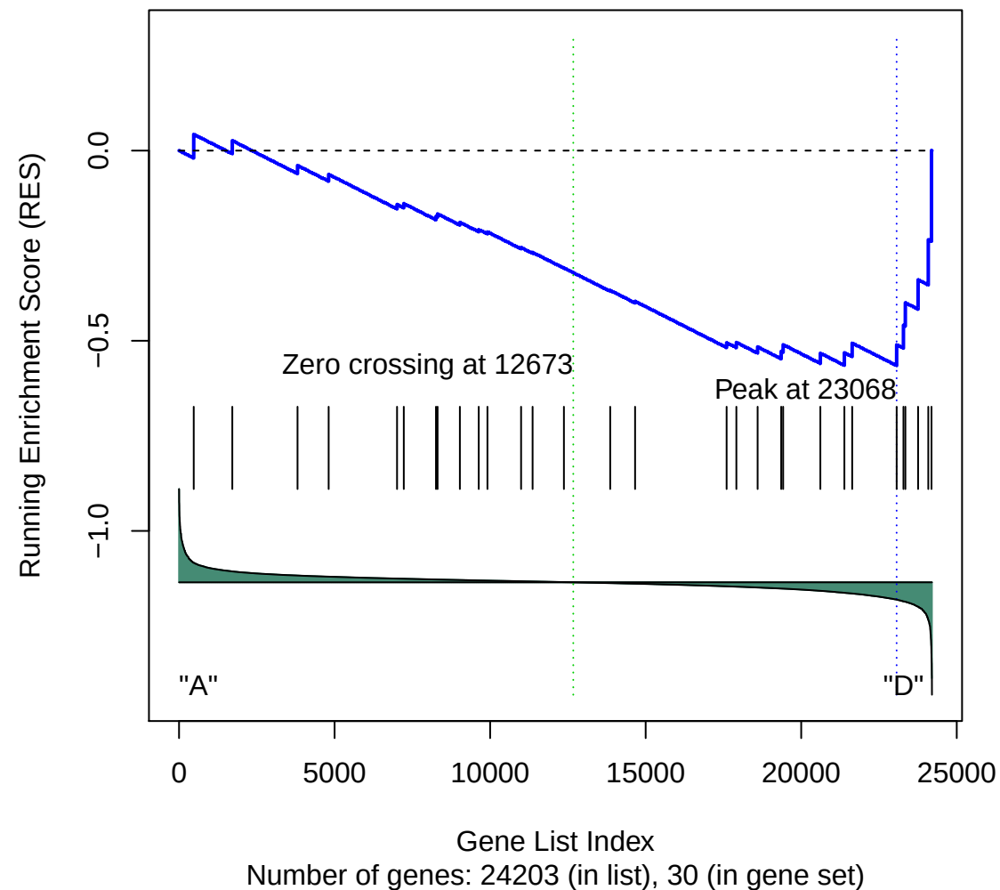
Gene Set 52 : KEGG_PROPANOATE_METABOLISM
