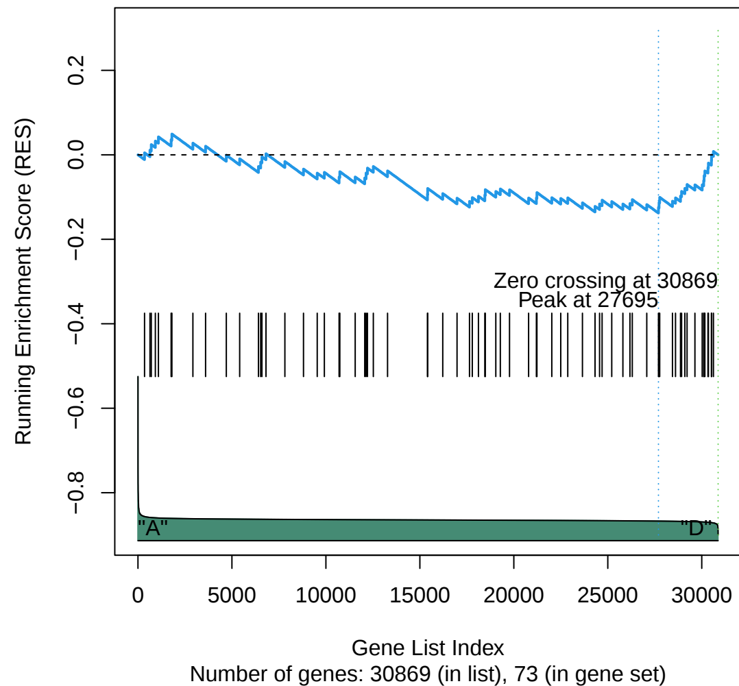
Gene Set 97 : KEGG_PEROXISOME
