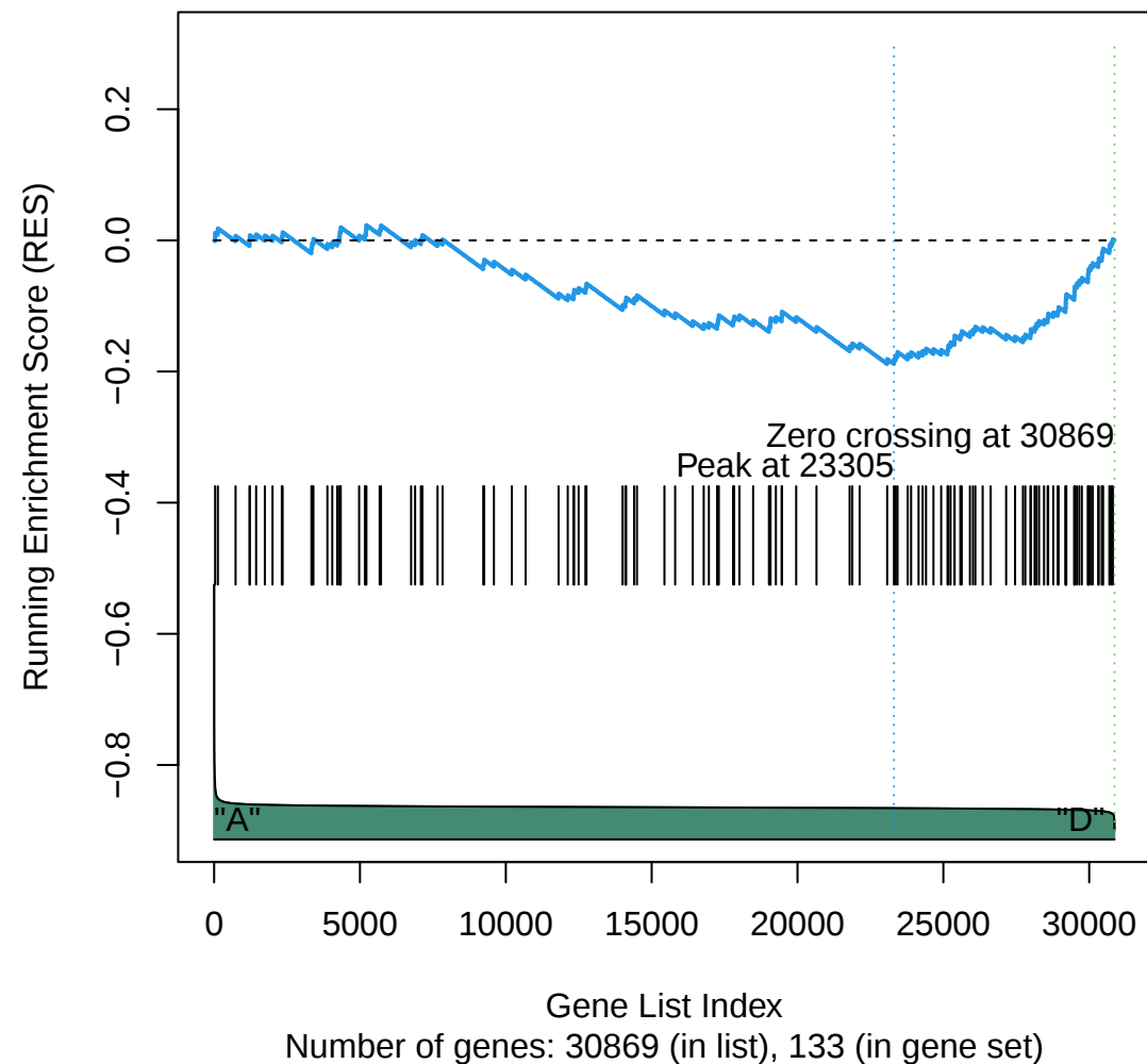
Gene Set 149 : KEGG_ALZHEIMERS_DISEASE
