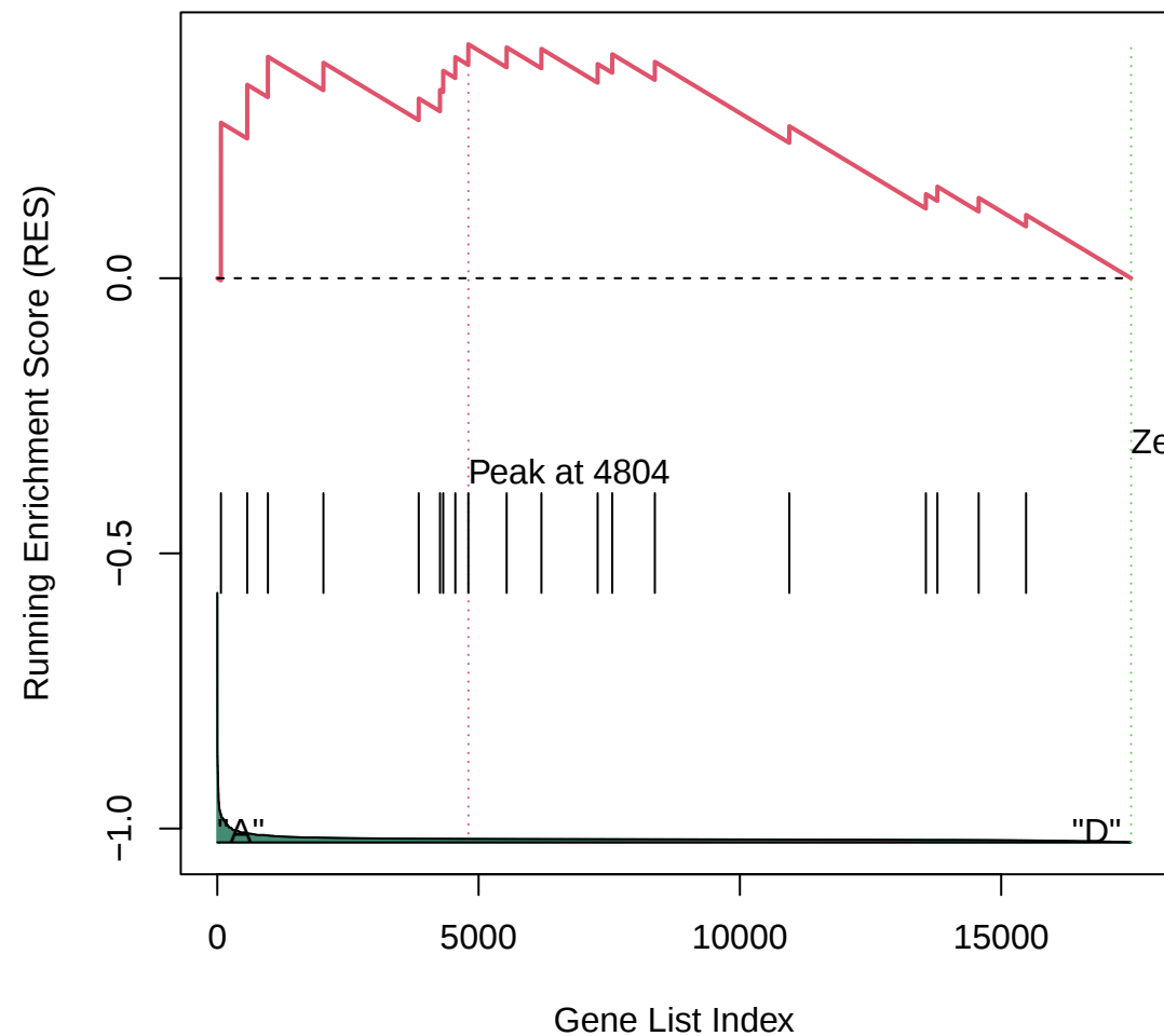
Gene Set 131 : KEGG_TASTE_TRANSDUCTION
